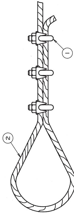
TYPICAL OF BOTH ENDS
