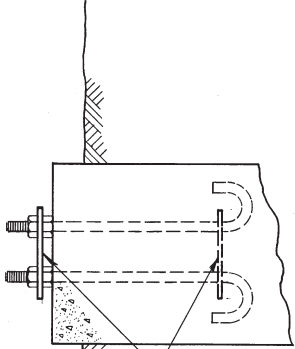
ANCHOR BOLT SETTING TEMPLATES (SEE CHART FOR PART NO. REQ'D.) REMOVE UPPER TEMPLATE BEFORE INSTALLING TOWER.
