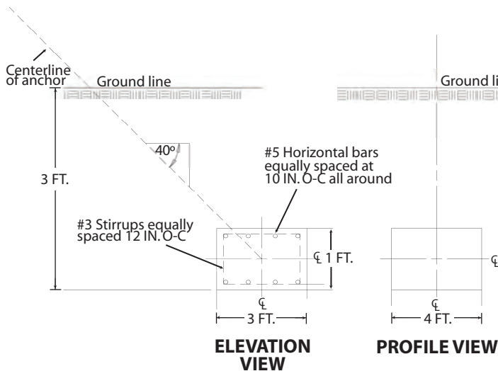
3E Concrete Volume 0.4 CU. YDS. per block 1.3 CU. YDS. total for 3
