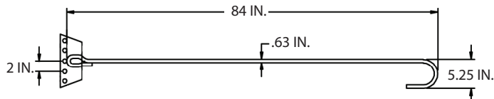
GAC305 ( 7,330 LBS. ALLOWABLE LOAD)*
