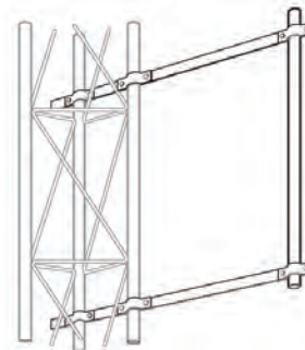
SIDE ARM BRACKET SA253UA
