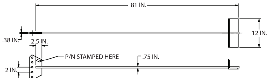
GAC3455TOP ( 17,670 LBS. ALLOWABLE LOAD)*
