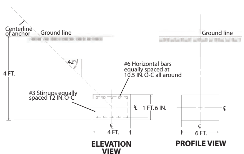
4E Concrete Volume 1.3 CU. YDS. per block 4.0 CU. YDS. total for 3
