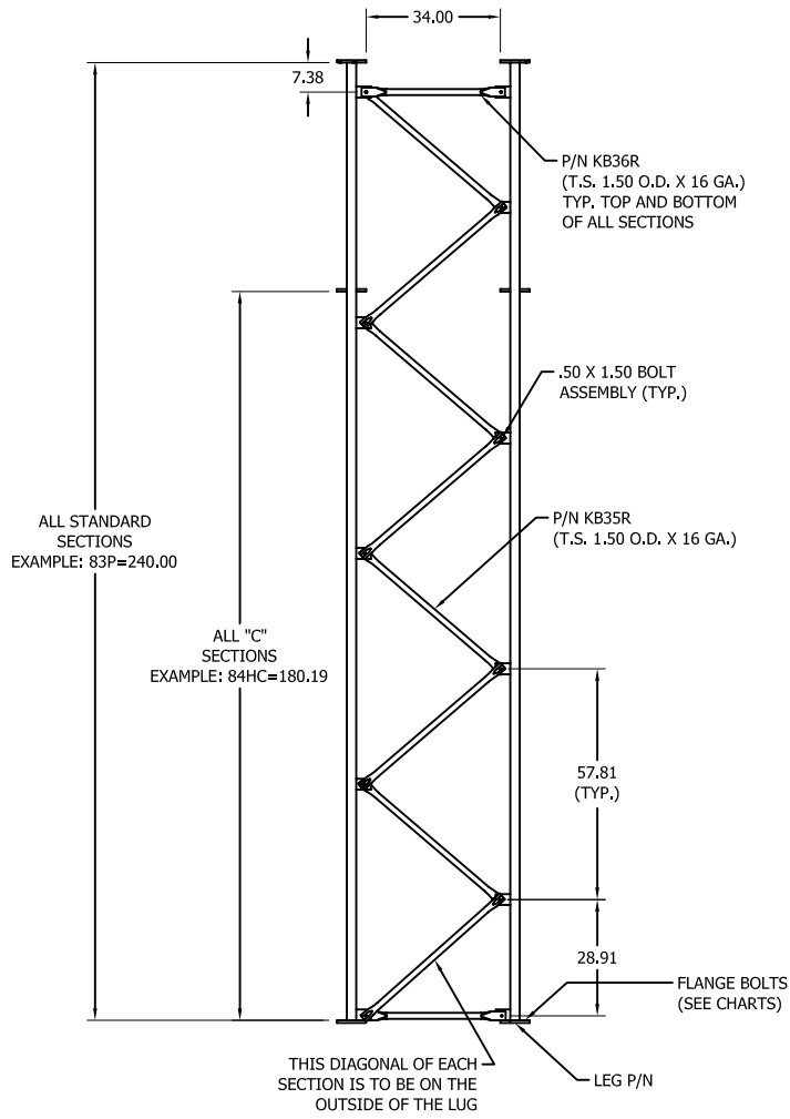
ELEVATION VIEW
