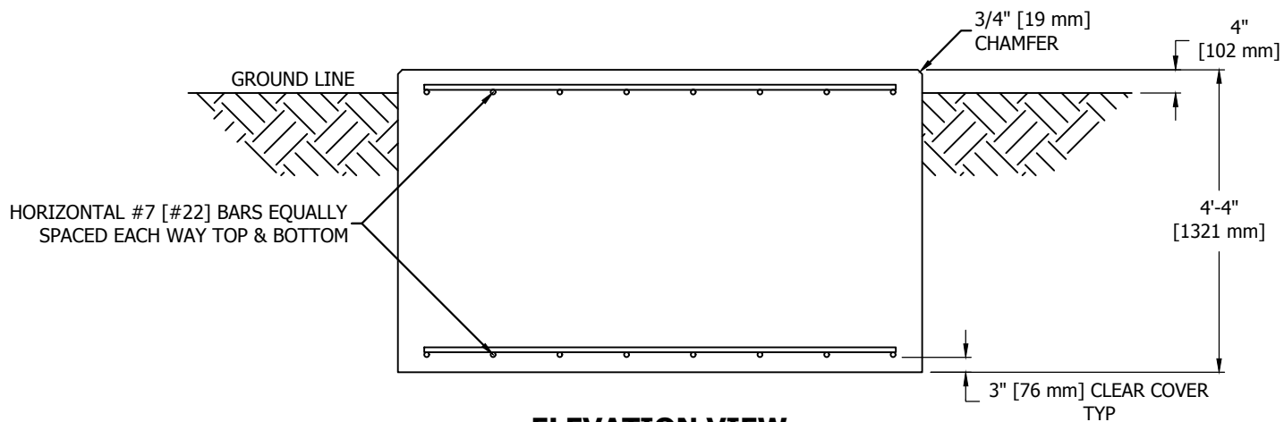
ELEVATION VIEW
