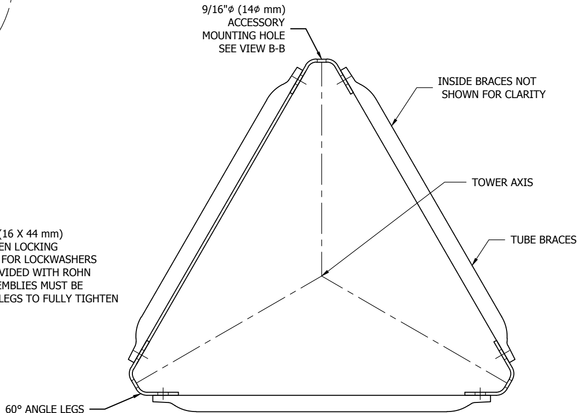
CROSS SECTION
