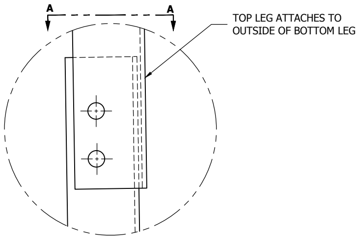
LEG SPLICE DETAIL
