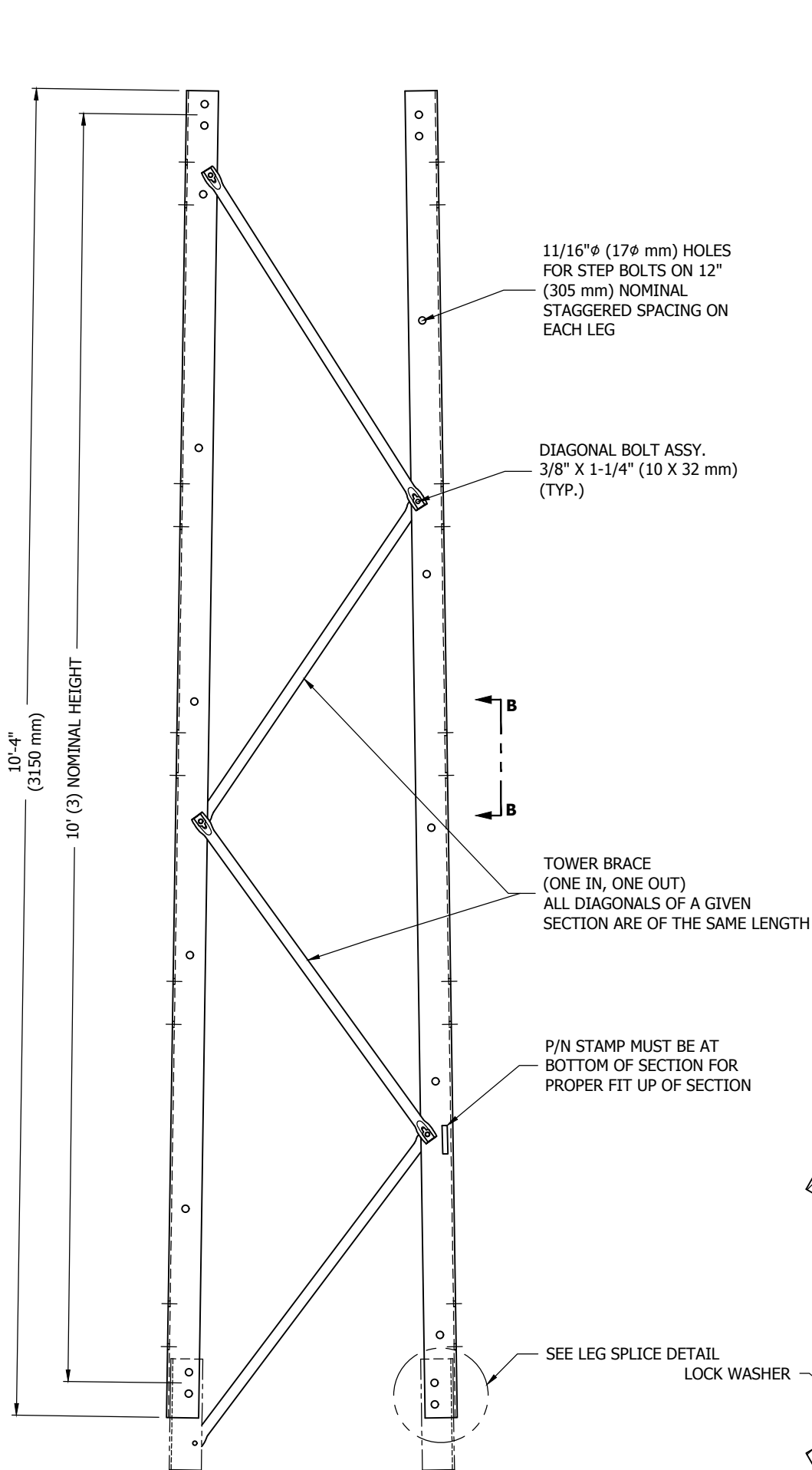
ELEVATION VIEW
